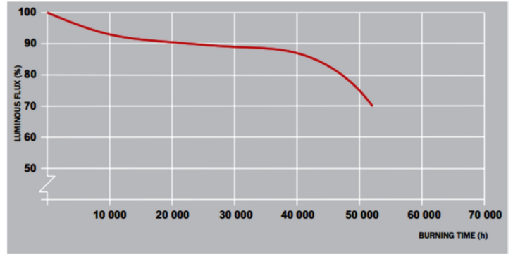
Service Life Aura T5 Eco Saver Long Life 3 h switching cycle (2 h 45 min. on, 15 min. off)
