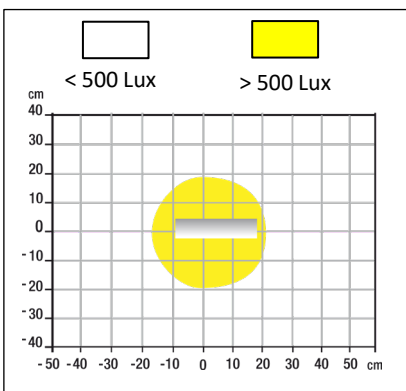
Measurement of Lux on the worktop in 35 cm top view:
